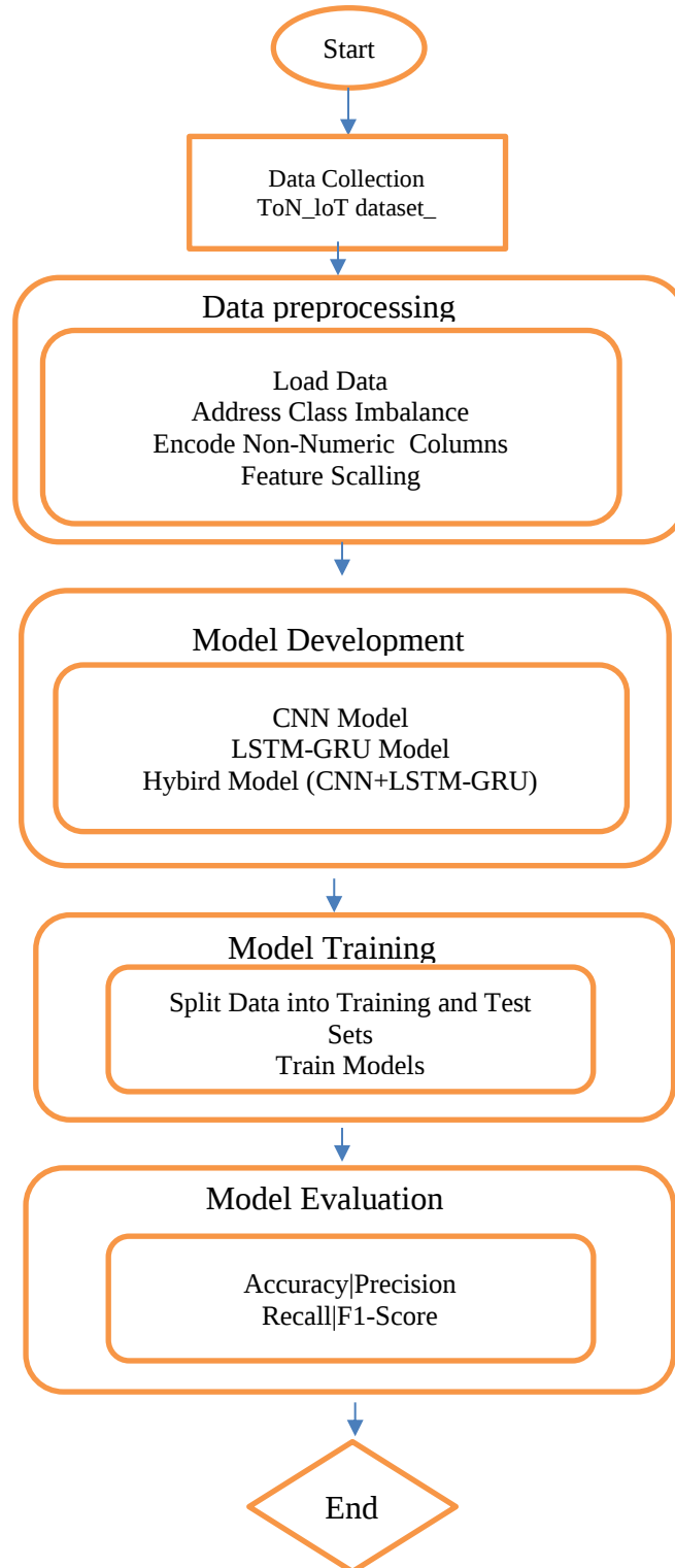
Figure 1. Proposed method
