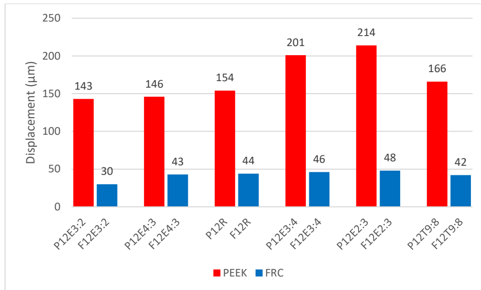
Figure (7): FEA reports the effect of two different framework materials on displacement(μm) for frameworks with a 12mm 2 sectional area
