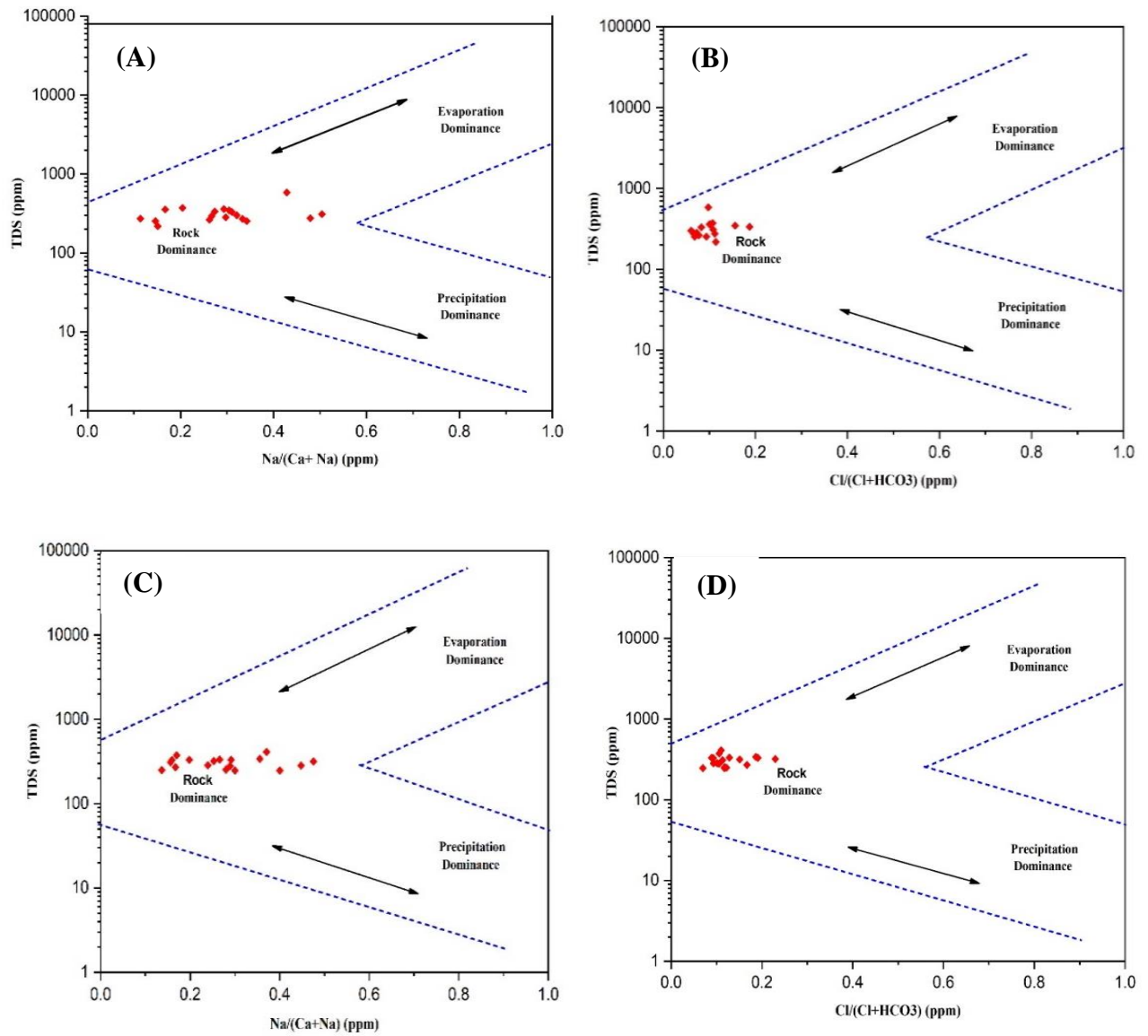
Fig.16. Mechanisms controlling groundwater quality (After Gibbs 1970) from the eastern part: (A, B) dry season (C, D) wet season
