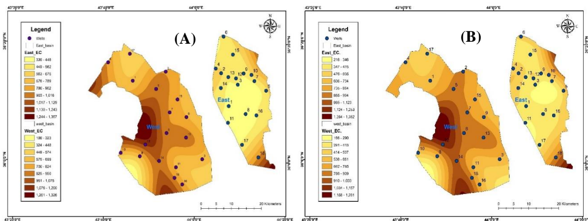
Fig. 4. Distribution of EC in the study area for: (A) dry season and (B) wet season
