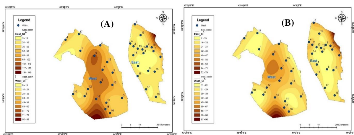
Fig. 14. Distribution of \text{Cl}^- in the study area for: (A) dry season, (B) wet season
