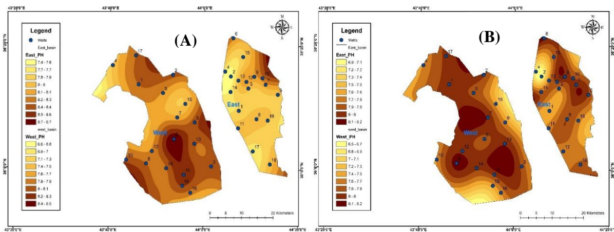
Fig. 3. Distribution of pH in the study area for: (A) dry season and (B) wet season
