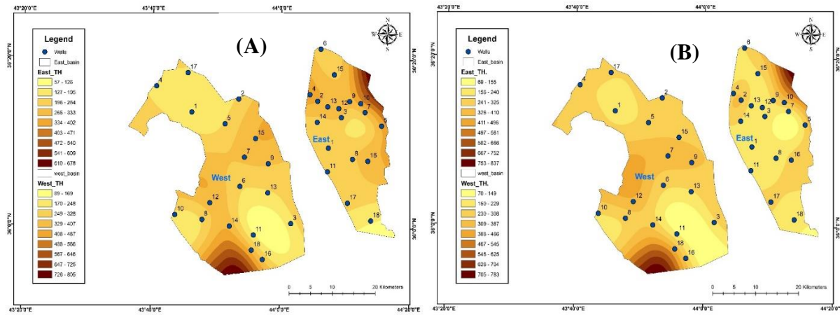
Fig. 11. Distribution of TH in the study area for: (A) dry season and (B) wet season
