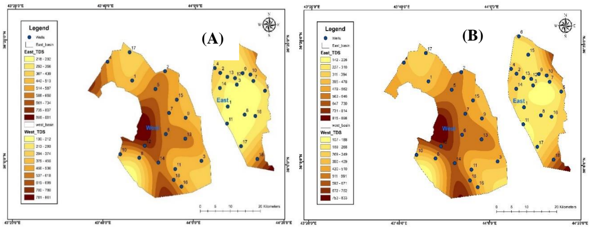
Fig. 5. Distribution of TDS in the study area for: (A) dry season and (B) wet season
