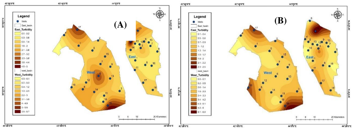
Fig. 6. Distribution of TU in the study area for: (A) dry season and (B) wet season
