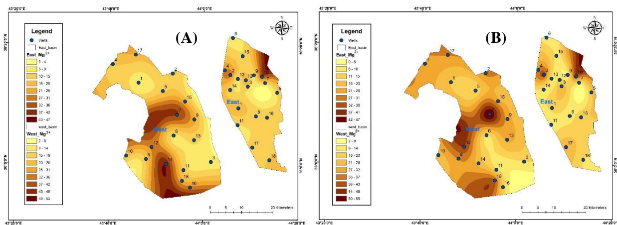
Fig. 8. Distribution of Mg^{2+} in the study area for: (A) dry season and (B) wet season
