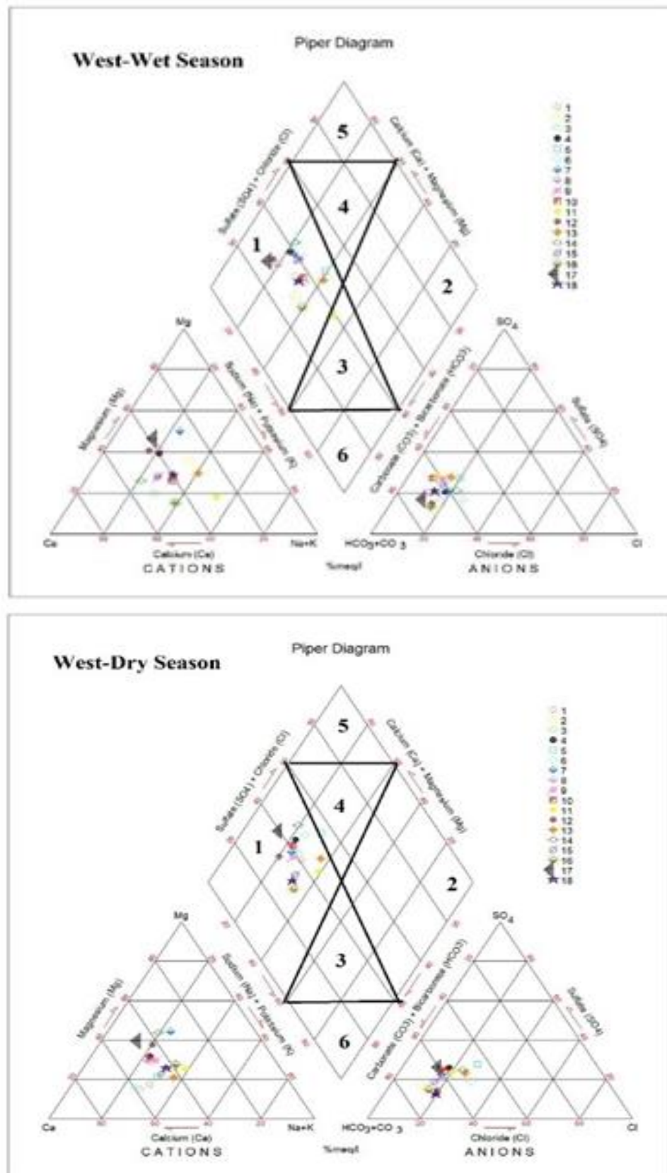
Fig. 19. Piper diagram depicting hydrochemical facies in dry and wet seasons from the western part of Erbil Basin
