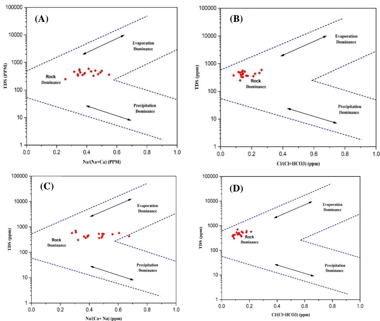
Fig.17. Mechanisms controlling groundwater quality (After Gibbs 1970) from the western part: (A, B) dry season (C, D) wet seas
