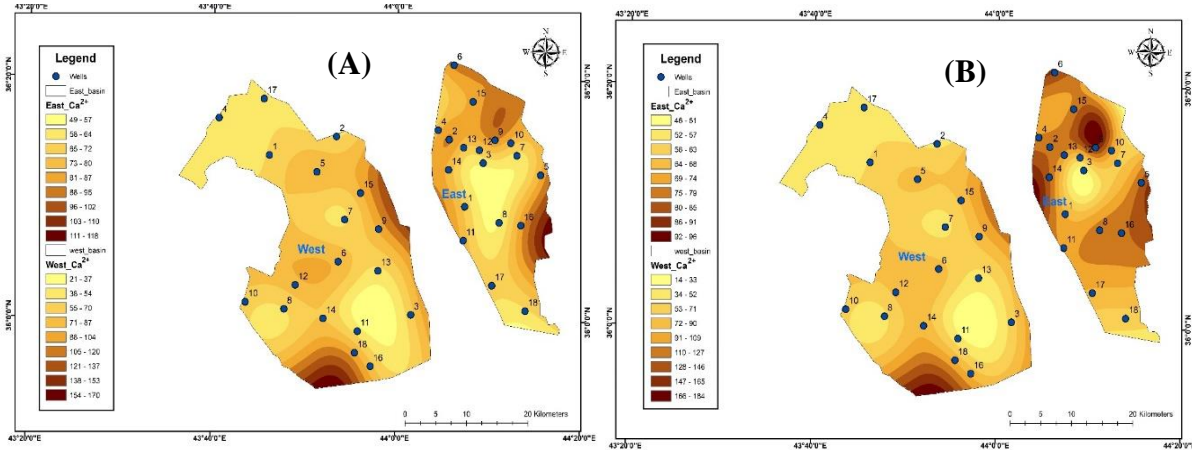
Fig. 7. Distribution of \text{Ca}^{2+} in the study area for: (A) dry season, (B) wet season
