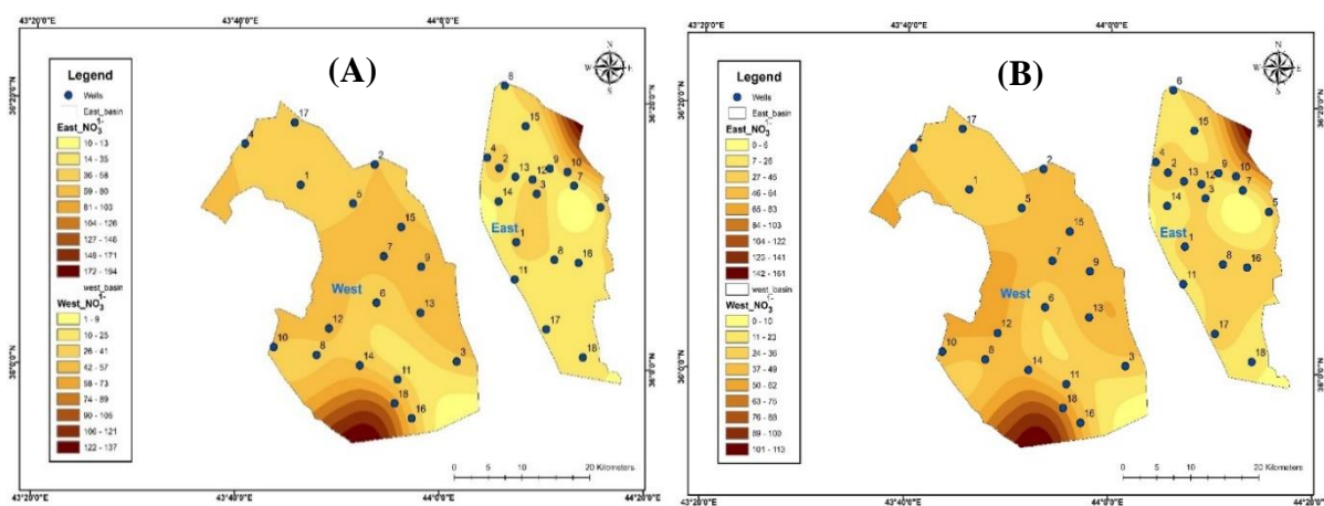
Fig. 15. Distribution of \text{NO}_3^- in the study area: (A) dry season and (B) wet season
