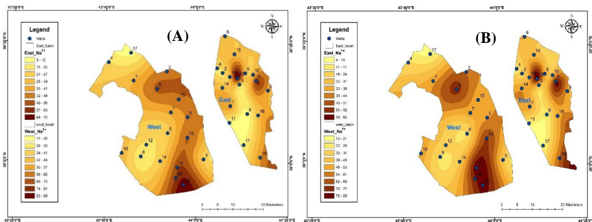
Fig. 9. Distribution of Na^{+} in the study area for: (A) dry season and (B) wet season
