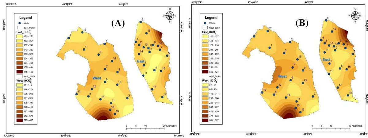
Fig. 12. Distribution of \text{HCO}_3^- in the study area for: (A) dry season and (B) wet season
