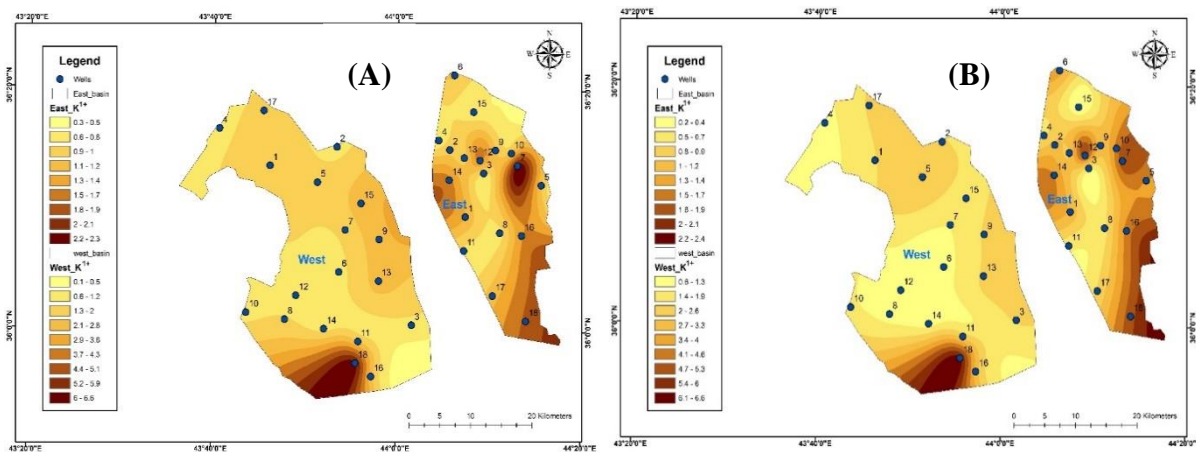
Fig. 10. Distribution of K^{+} in the study area for: (A) dry season and (B) wet season
