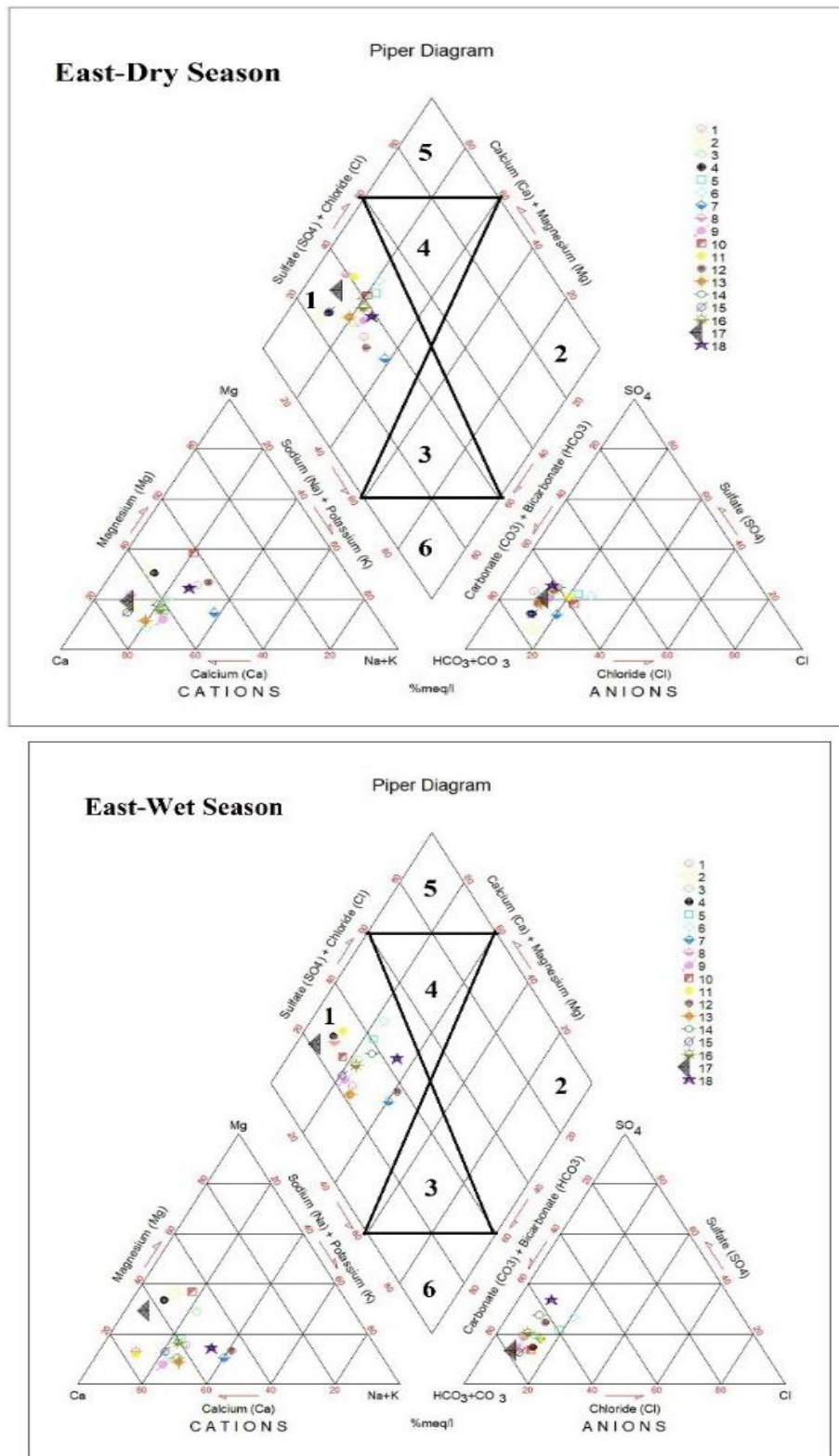
Fig. 18. Piper diagram depicting hydrochemical facies in dry and wet seasons from the eastern part of Erbil Basin
