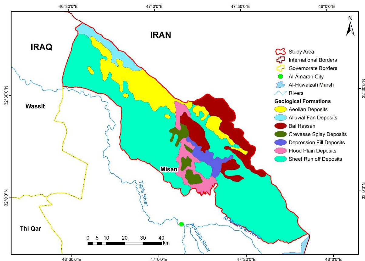
Fig. 8. Geological formations in the study area.
