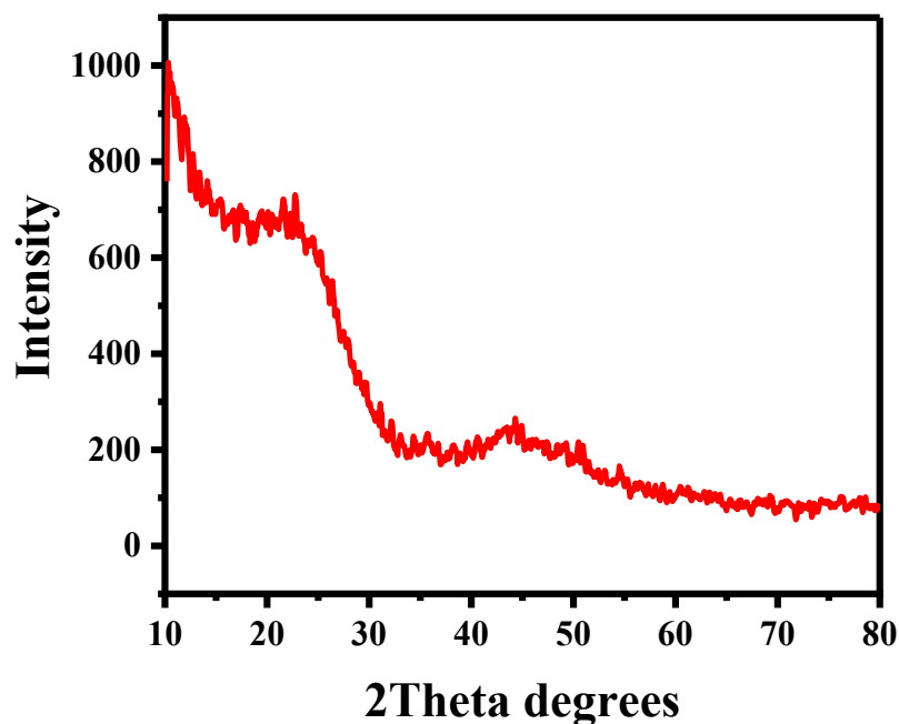
Figure 4. XRD image of NSAC
