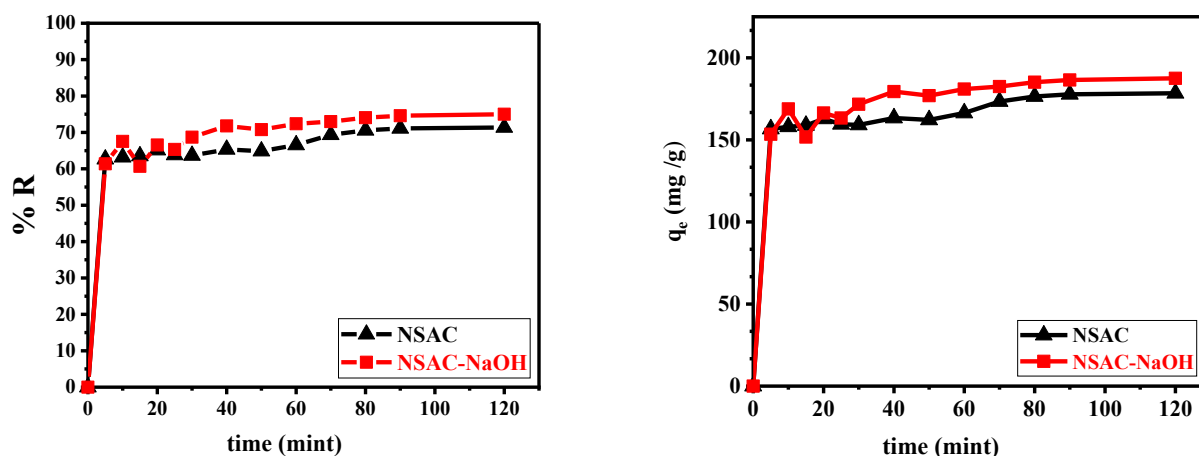
Figure 7. Effect of contact time on the adsorption of EBT on NSAC and NSAC-NaOH at 25 °C
