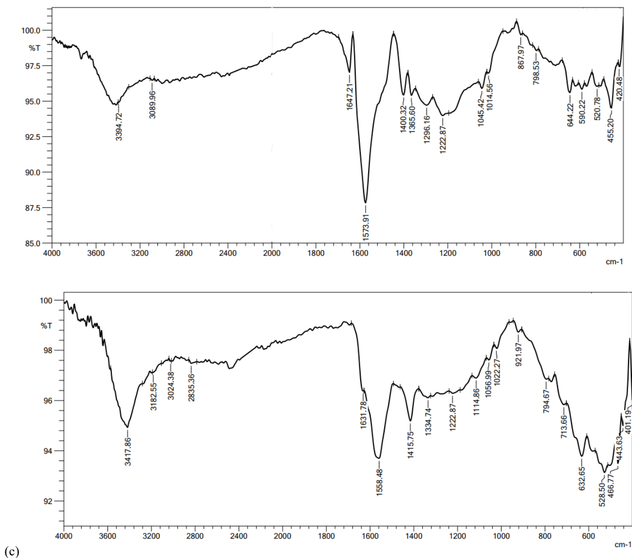
Figure 1. FT-IR spectra for (a) NSAC before adsorption, (b) NSAC after adoption, and (c) NSAC-NaOH
